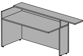
Right Recessed Leg + Extended 38"H Transaction Top
