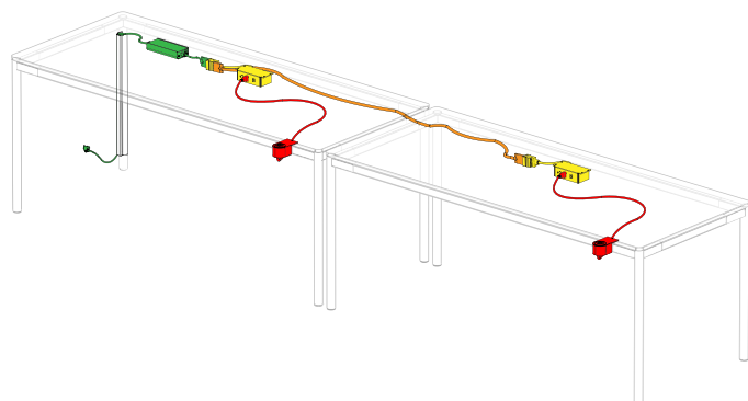
C. Daisy-chained Power between 2 Tables
