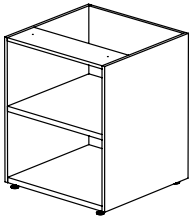
PSP0 | Pedestal Open Style
